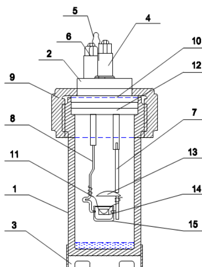
Fig. 1. Bomb calorimeter
